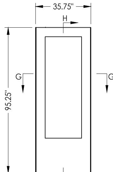
FIBERGLASS DOOR PANEL Therma Tru 8"
