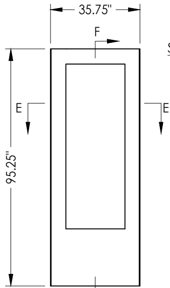
FIBERGLASS DOOR PANEL Plastpro 8"
