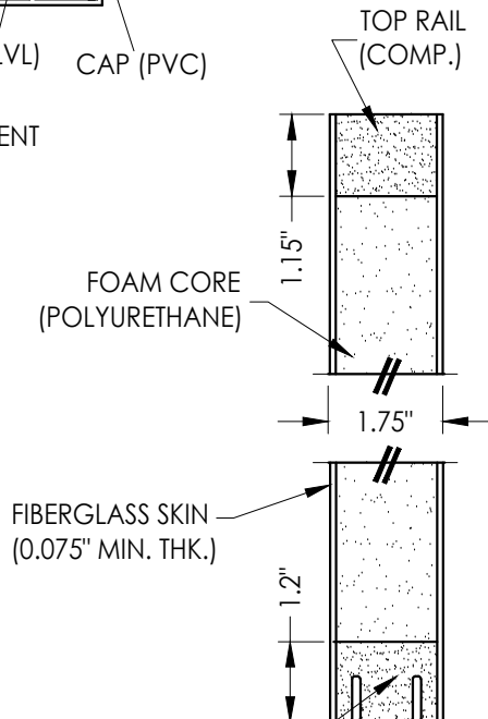
SECTION F-F
