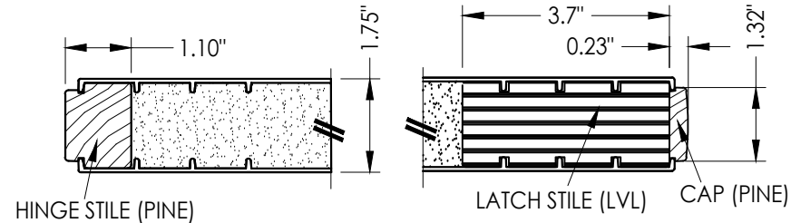
SECTION G-G
