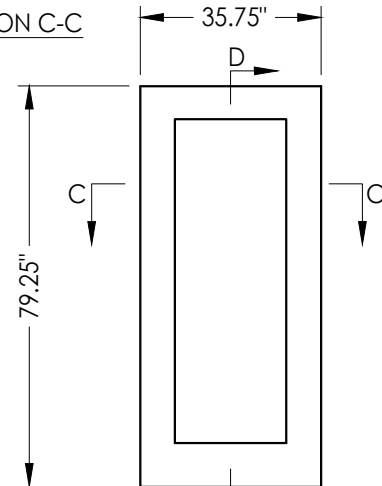
FIBERGLASS DOOR PANEL Therma Tru 6' 8"
